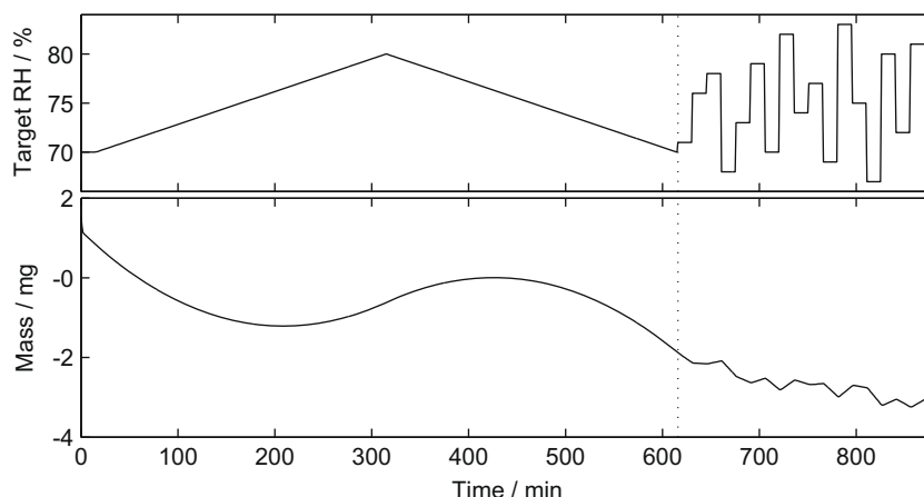
Fig. 1. The RH programs and the measured mass for NaCl. The vertical dashed line shows when the ramp method ends and the step method starts.
