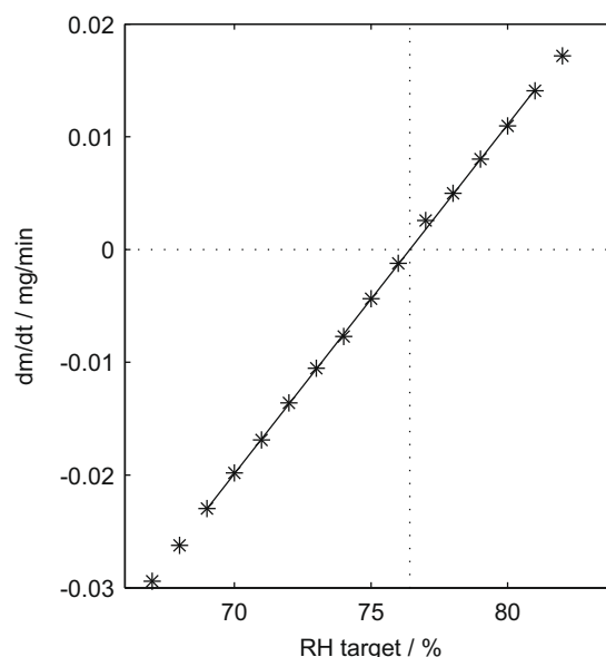
Fig. 4. Evaluation of the step method for NaCl. Each point is the dm/dt calculated for one RH step. The dashed lines indicate how the RH was evaluated.
