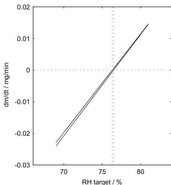
Fig. 3. Evaluation of the ramp method for NaCl. Data points and linear regression are shown for absorption and desorption. The dotted lines indicate how the RH was evaluated.
