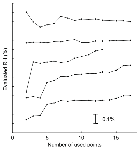
Fig. 5. The RH evaluated from the RH-steps using different number of data points. From top to bottom the curves refer to the following runs: LiCl (20 °C), NaCl (25 °C), MgCl 2 (25 °C), Mg(NO 3 ) 2 (25 °C), and Mg(NO 3 ) 2 (20 °C).
