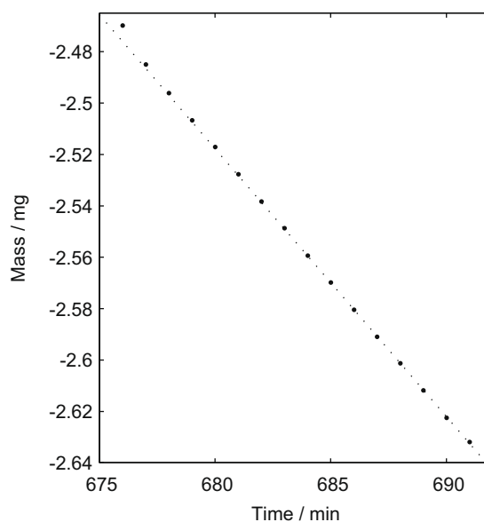
Fig. 2. Detail showing the mass during a typical 15 min RH step for the NaCl validation shown in Fig. 1. The mass change rate was evaluated with linear regression of all data points on the second half of the step.
