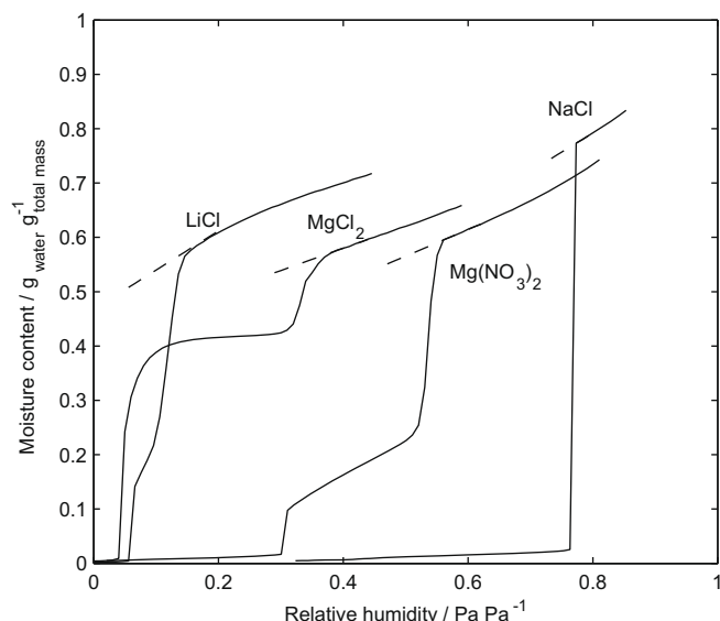
Fig. 6. Sorption isotherms measured with a sorption microcalorimeter at 25 °C for the four used salts. The slopes of interest are indicated by dotted lines. Note that because of kinetic effects, the deliquescence steps are not perfectly vertical as they should be. Note also that MgCl 2 and Mg(NO 3 ) 2 show the formation of hexa-hydrates at lower RH than deliquescence (for MgCl 2 this step does not correspond to the full anhydrous to hexa-hydrate transformation as this salt was not completely dried before the measurements).
